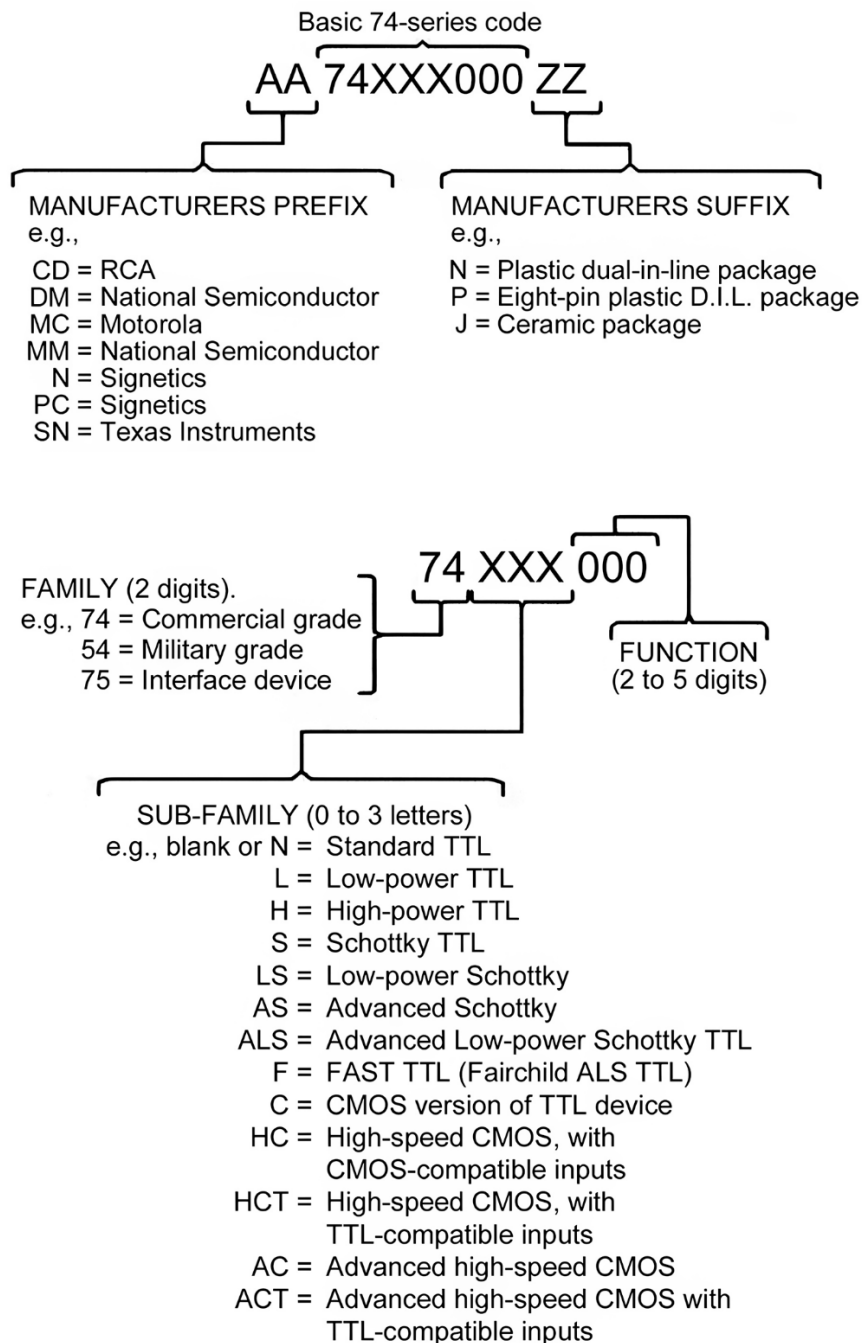
Fig 1: Interpretation of 74-series logic IC codes
